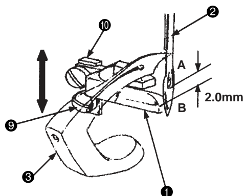
Vertical direction of rear needle guide
