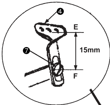
Standard dimension
