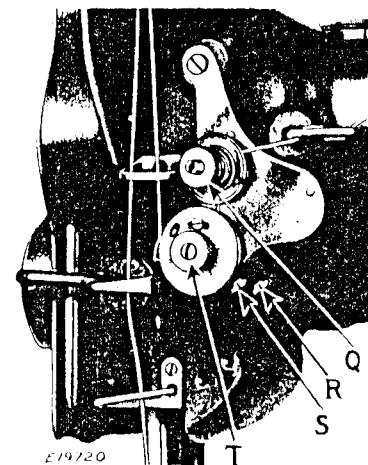
Fig. 21. Adjustments on Thread Controller
